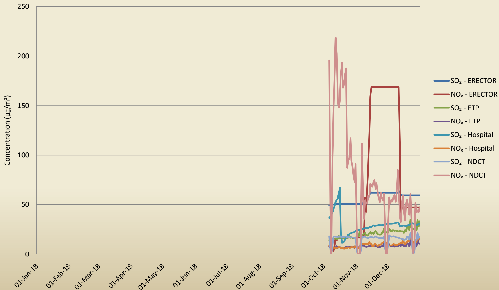
Annual Ambient Trend of Gaseous in M/s. Satpuda Thermal Power Station, Dist. Betul (M.P.)
